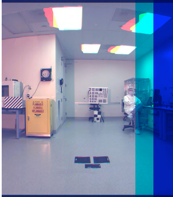
Fig. 25 This color image mosaic was taken with \text{TDI} = 4 while Junocam was moving at the nominal rate of 2 RPM. Residual color artifacts are from uncorrected parallax effects and sensor blooming from direct imaging of the overhead lights. This image would have been blurred if TDI had been implemented incorrectly
