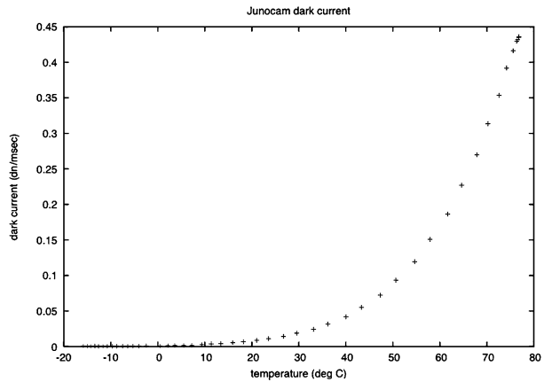
Fig. 20 Dark current as a function of temperature has been measured. The camera temperature at Jupiter will range between -26^{\circ}\text{C} and +11^{\circ}\text{C}
