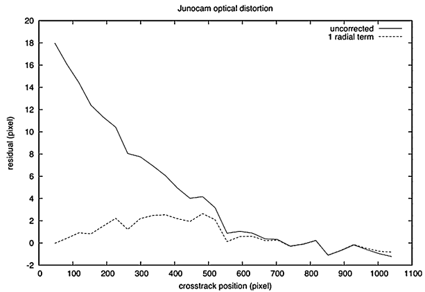
Fig. 23 Residuals between actual pixel measurements of a dot target and camera models are shown. The solid line uses the function for an ideal pinhole lens; the dashed line uses a model incorporating a radial distortion
